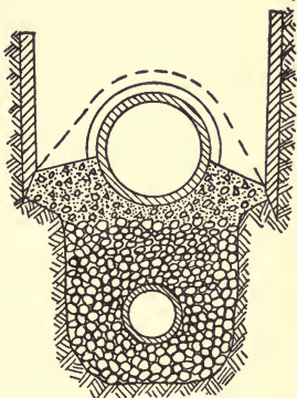
FIG. 27.—SEWER-PIPE LAID IN CONCRETE.
